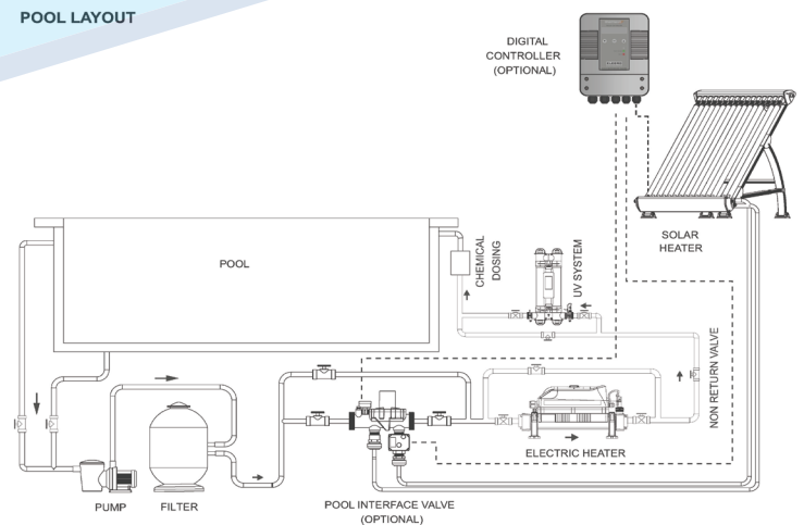
POOL LAYOUT
